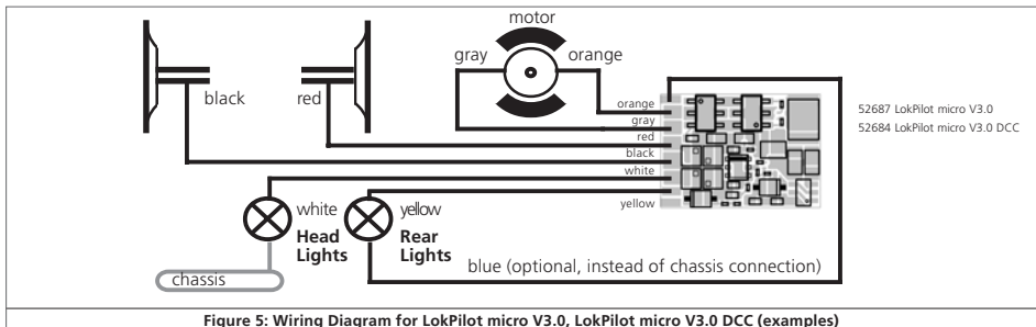
Figure 5: Wiring Diagram for LokPilot micro V3.0, LokPilot micro V3.0 DCC (examples)
